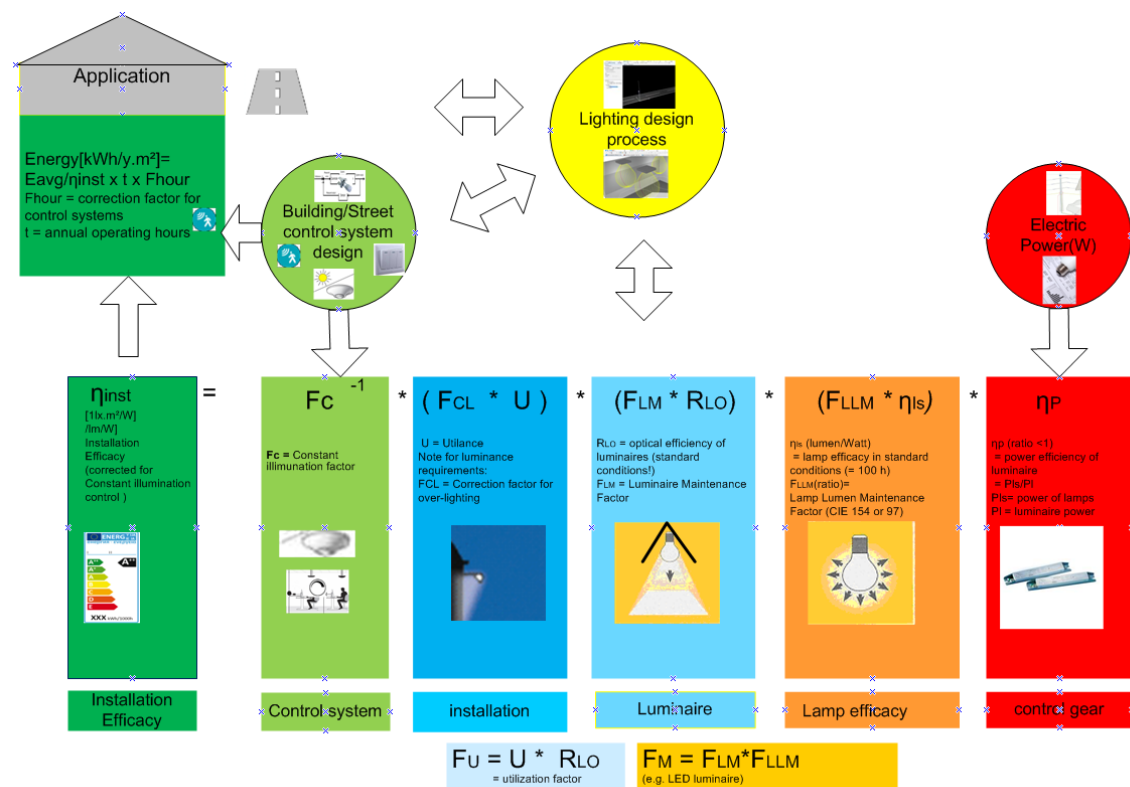
Figure 10: Components of a lighting system and the most relevant performance parameters related to energy efficiency
